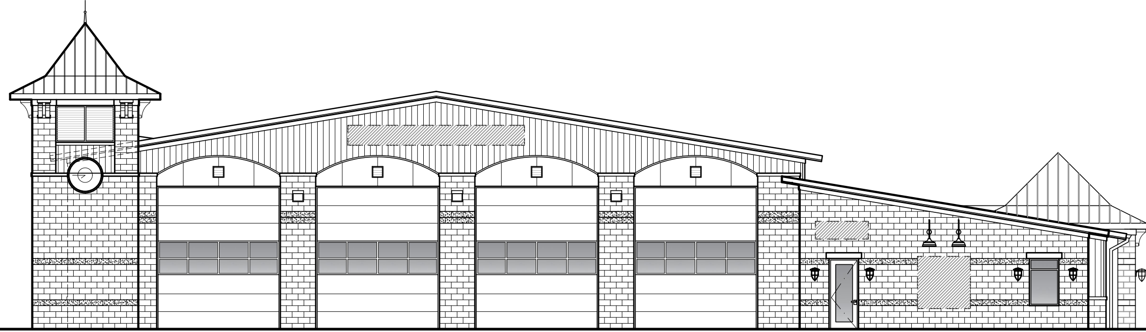
NORTH ELEVATION 2 SCALE: 3/32" = 1'-0" A-2
